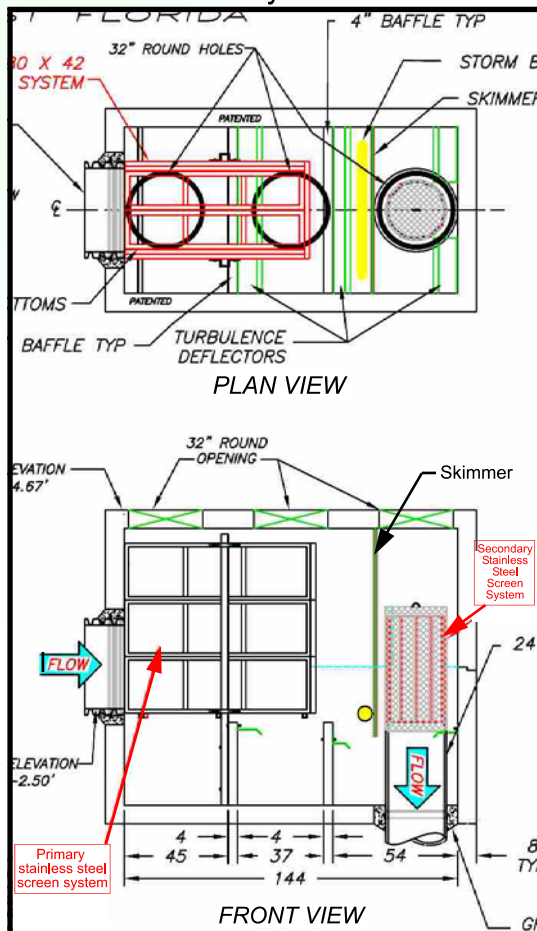
Schematic of Key West Structures
