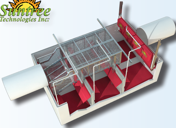
NSBB™ with HydroSlide® (Optional)
